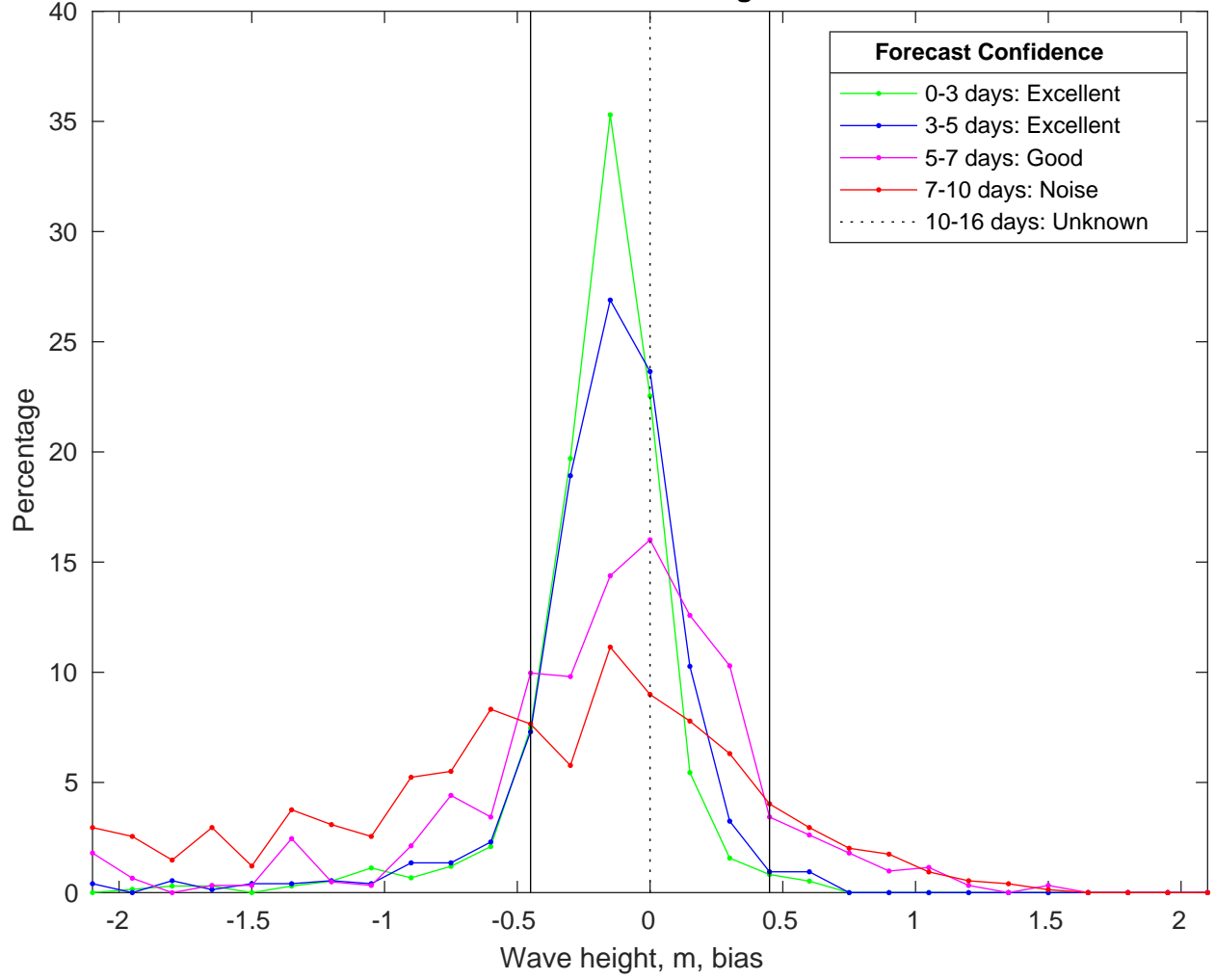
NDBC 42040 vs CMEMSWaves Bias Histogram: 21-Jan-2025
