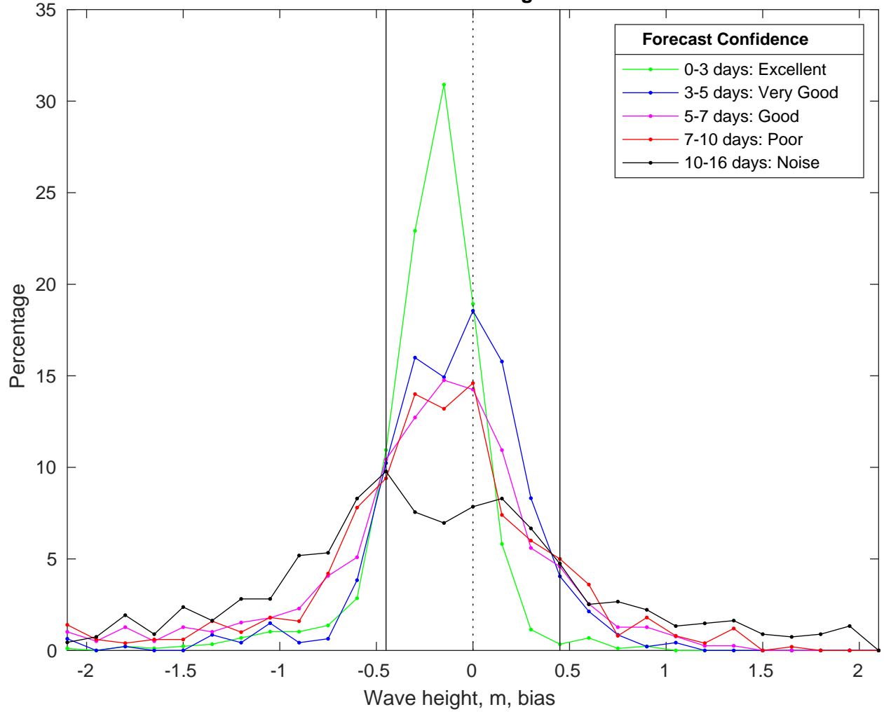
NDBC 42040 vs GFSWaves Bias Histogram: 21-Jan-2025
