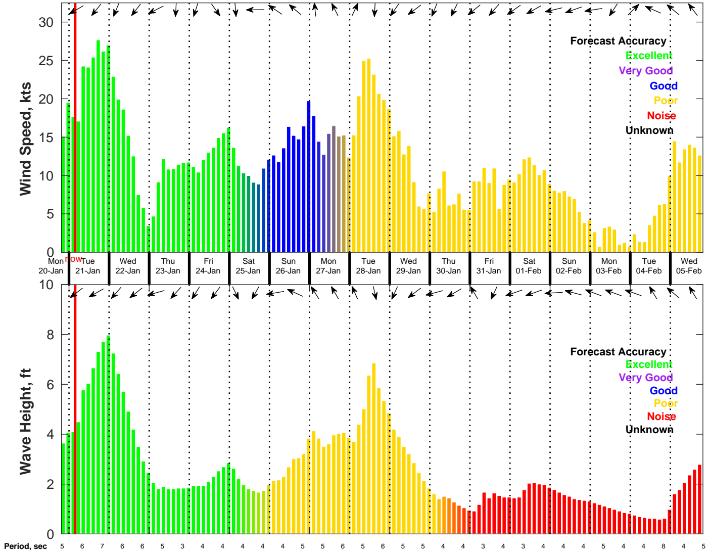
Wind & Wave Forecast for NDBC 42040 from 20-Jan-2025 19:00:00 to 05-Feb-2025 19:00:00
