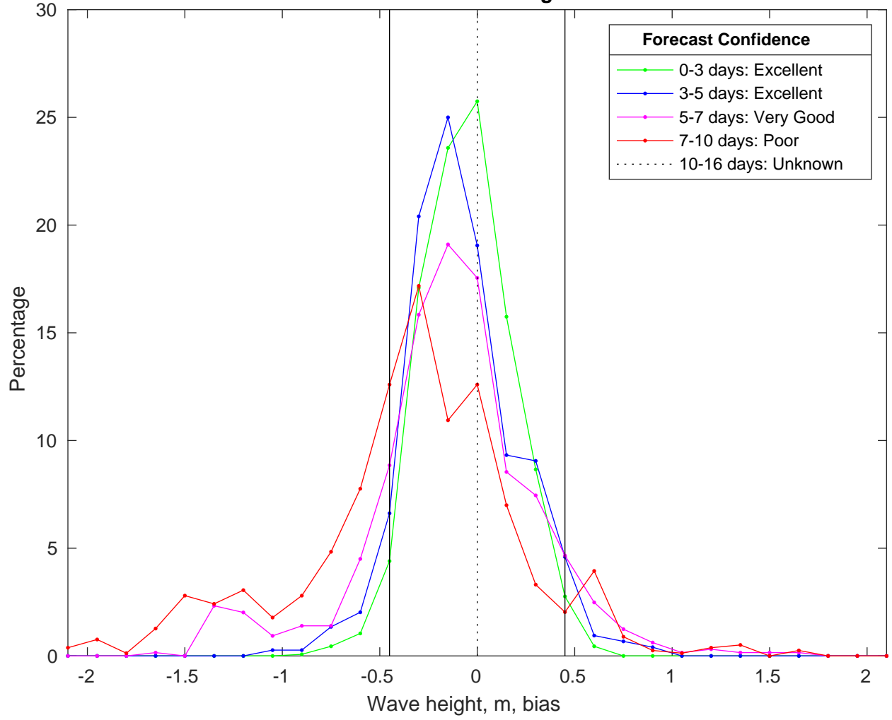
NDBC 42084 vs CMEMSWaves Bias Histogram: 21-Jan-2025
