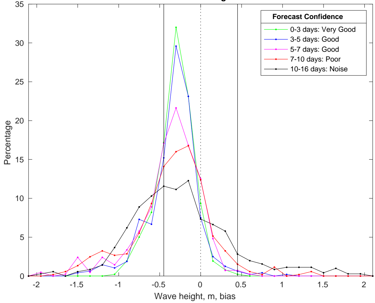
NDBC 42084 vs GFSWaves Bias Histogram: 21-Jan-2025
