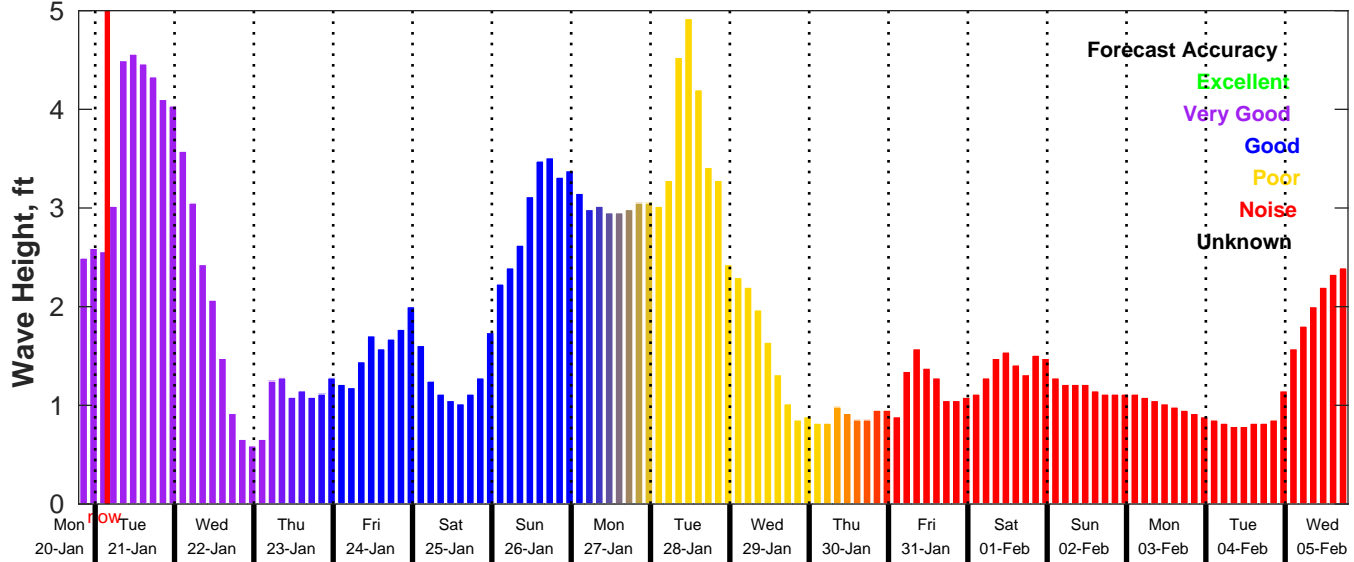
GFS Wave Forecast for NDBC 42084 from 20-Jan-2025 19:00:00 to 05-Feb-2025 19:00:00
