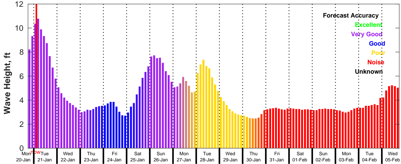
GFS Wave Forecast for NDBC 42092 from 20-Jan-2025 18:00:00 to 05-Feb-2025 18:00:00
