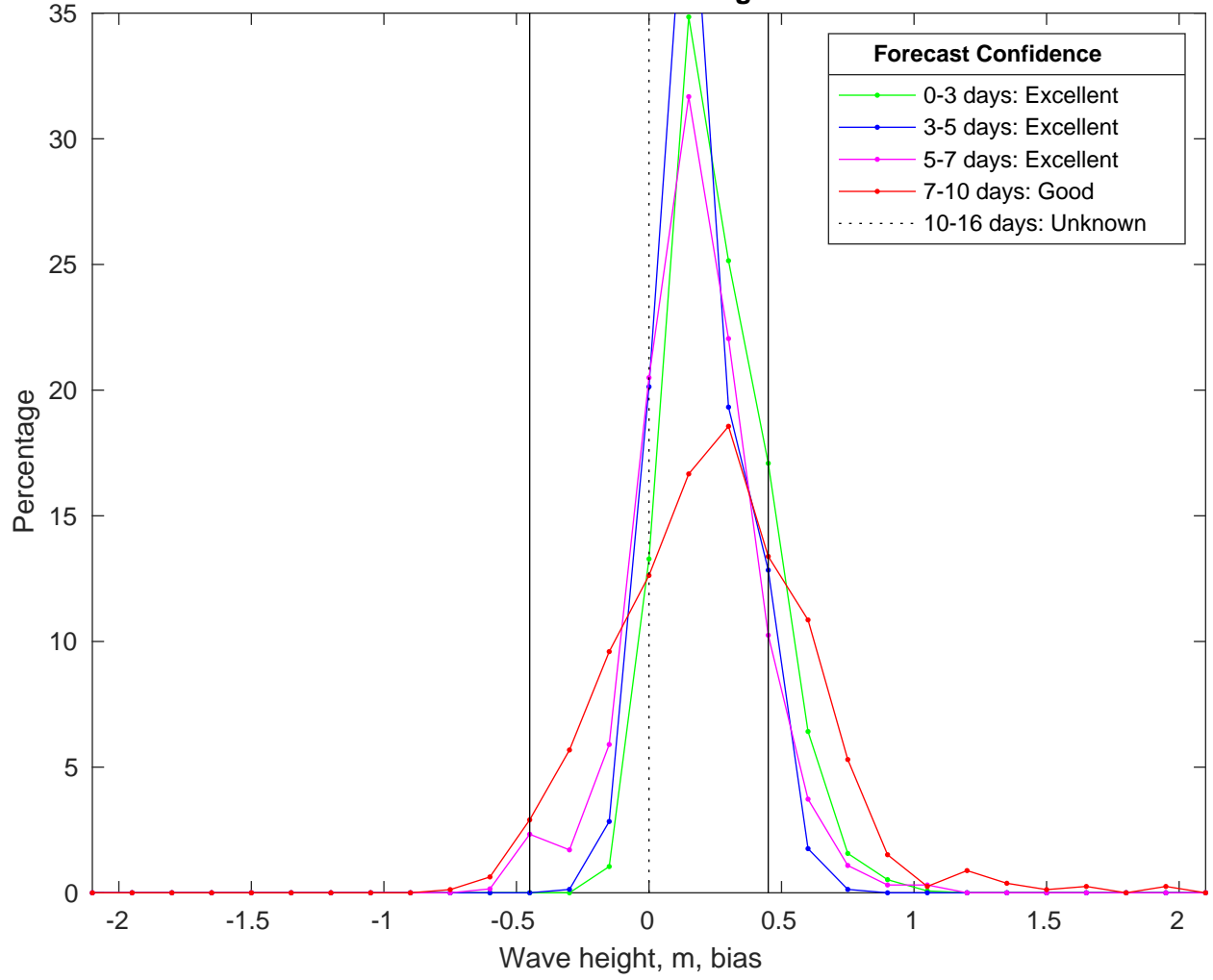
NDBC 44020 vs CMEMSWaves Bias Histogram: 21-Jan-2025
