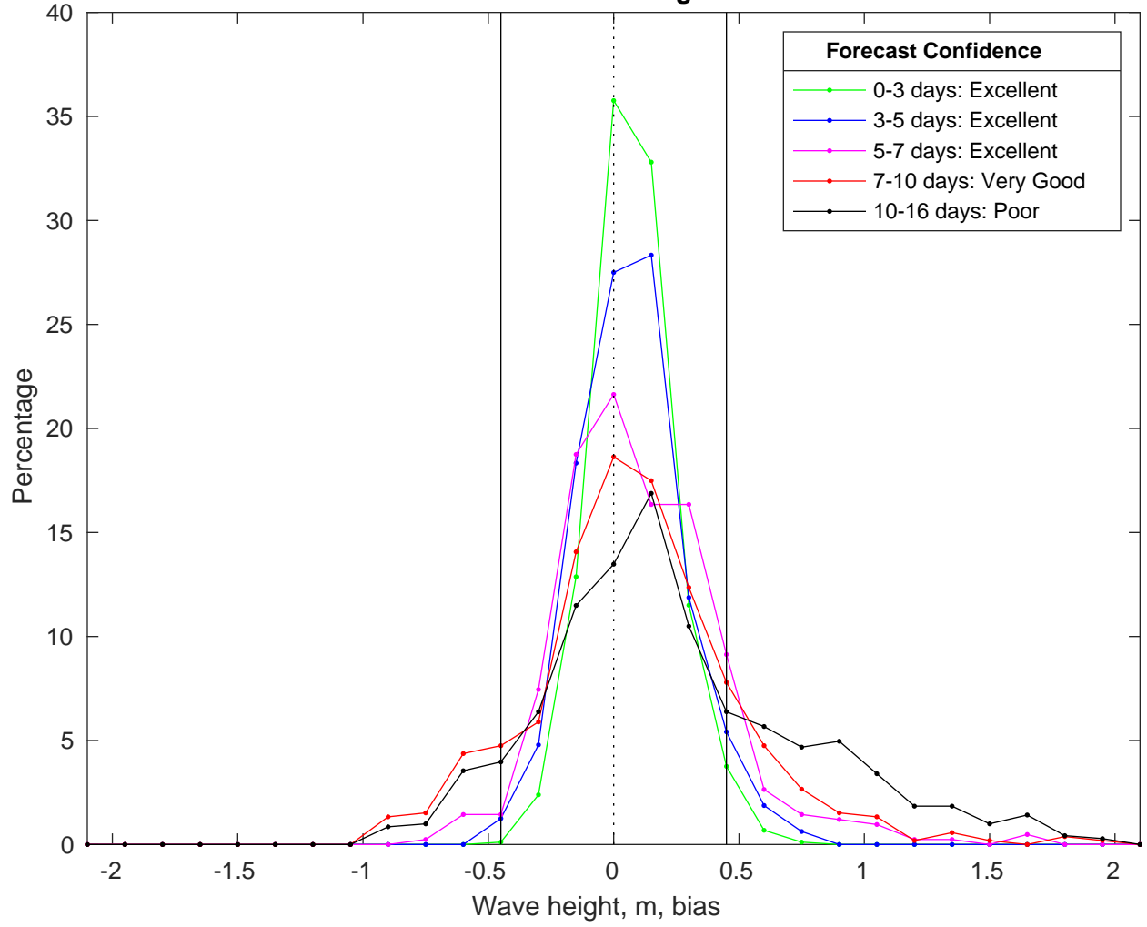
NDBC 44020 vs GFSWaves Bias Histogram: 21-Jan-2025
