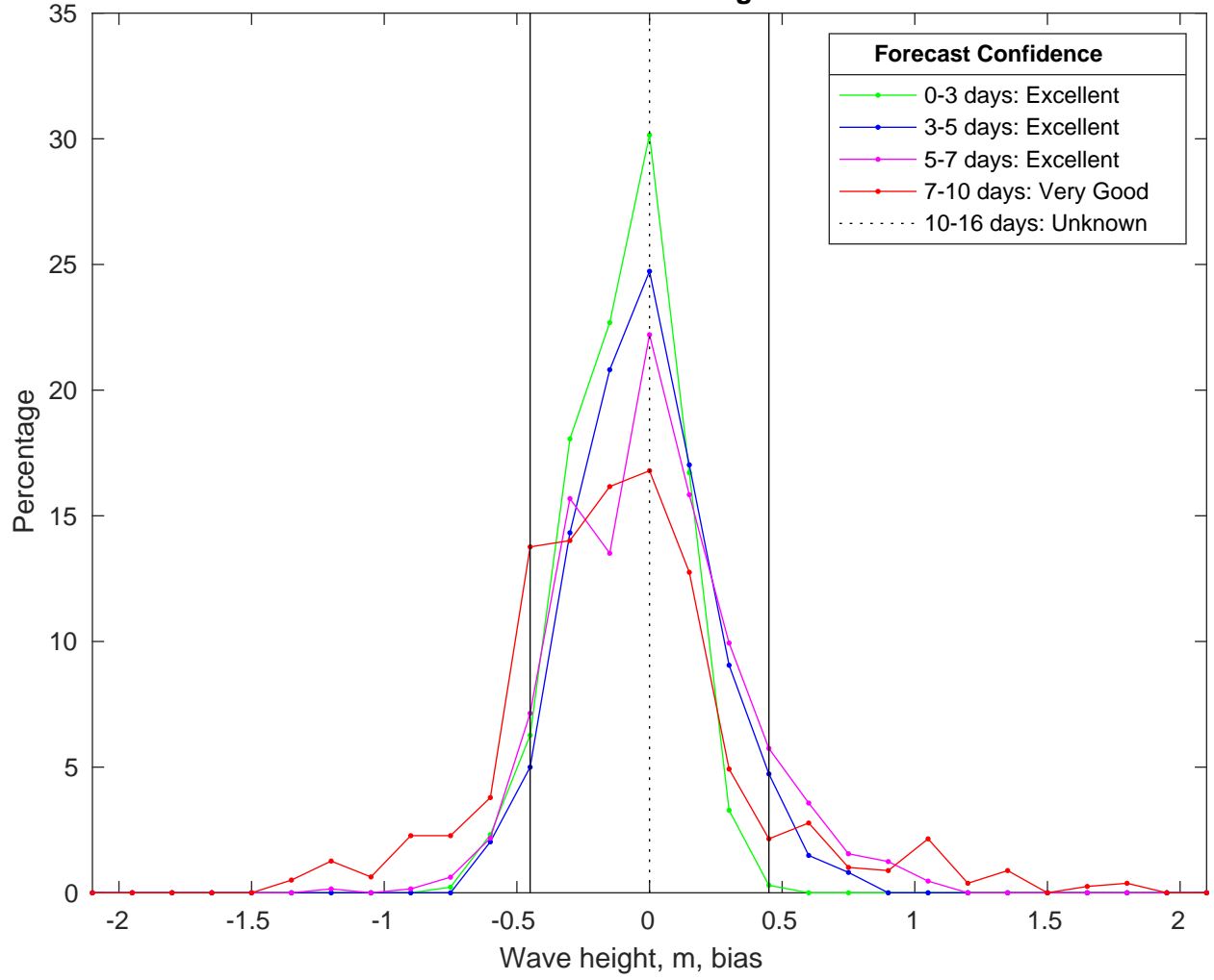
NDBC 46011 vs CMEMSWaves Bias Histogram: 21-Jan-2025
