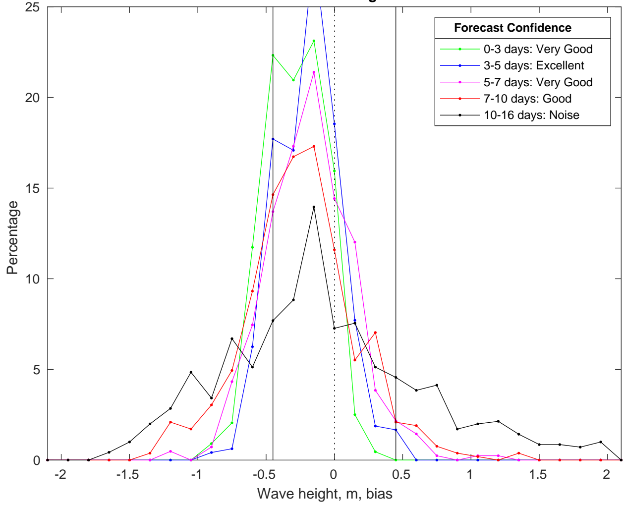
NDBC 46011 vs GFSWaves Bias Histogram: 21-Jan-2025
