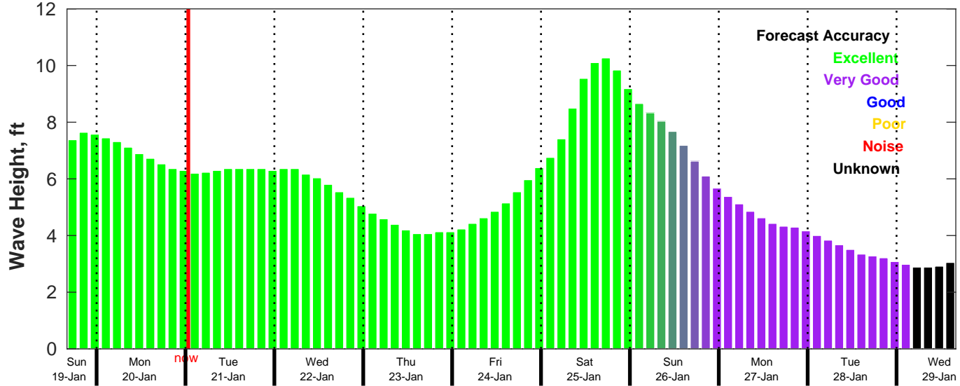
CMEMS Wave Forecast for NDBC 46011 from 19-Jan-2025 16:00:00 to 29-Jan-2025 16:00:00
