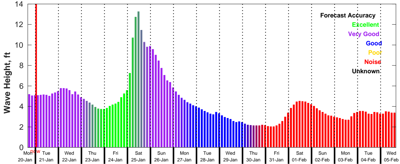
GFS Wave Forecast for NDBC 46011 from 20-Jan-2025 16:00:00 to 05-Feb-2025 16:00:00
