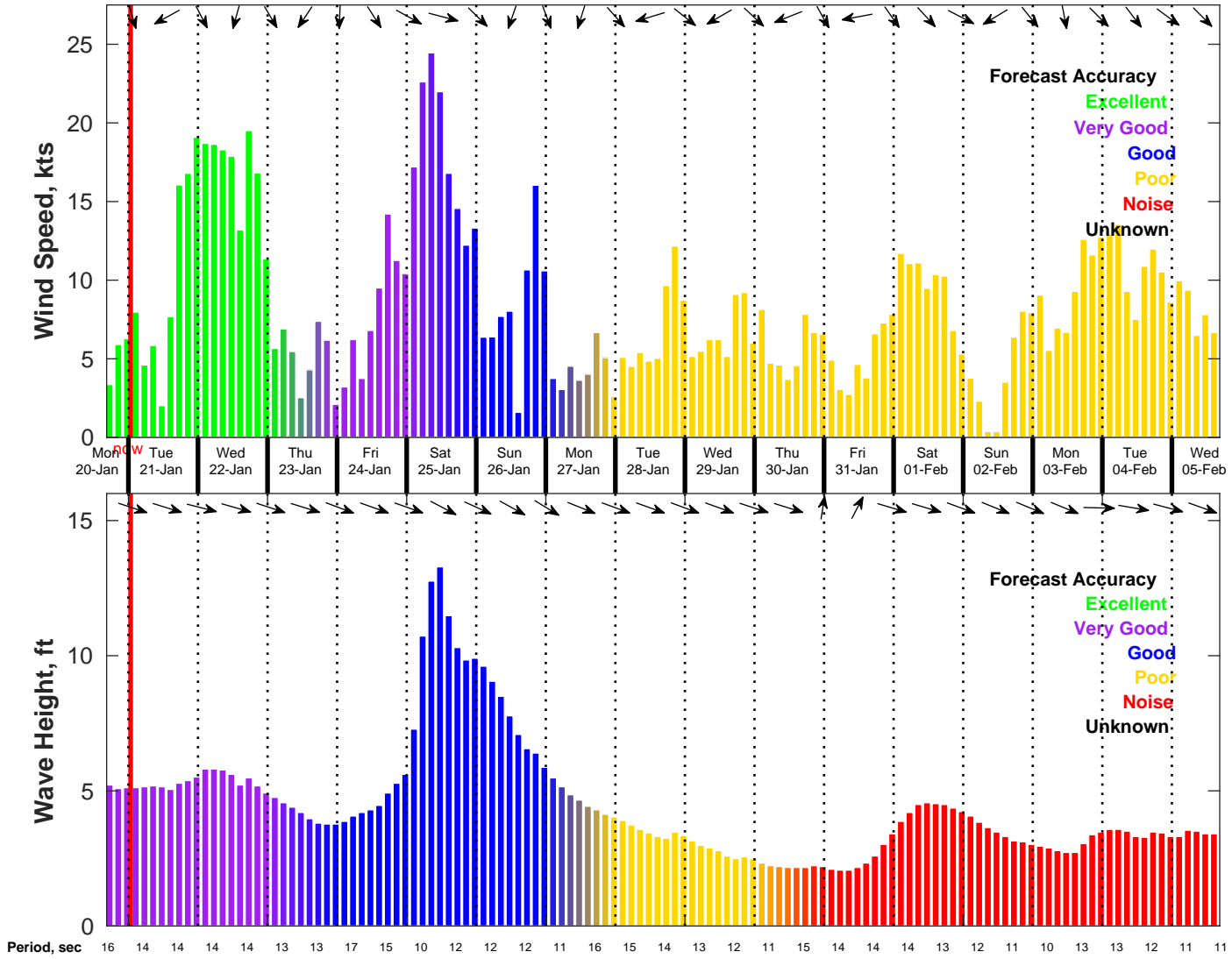
Wind & Wave Forecast for NDBC 46011 from 20-Jan-2025 16:00:00 to 05-Feb-2025 16:00:00
