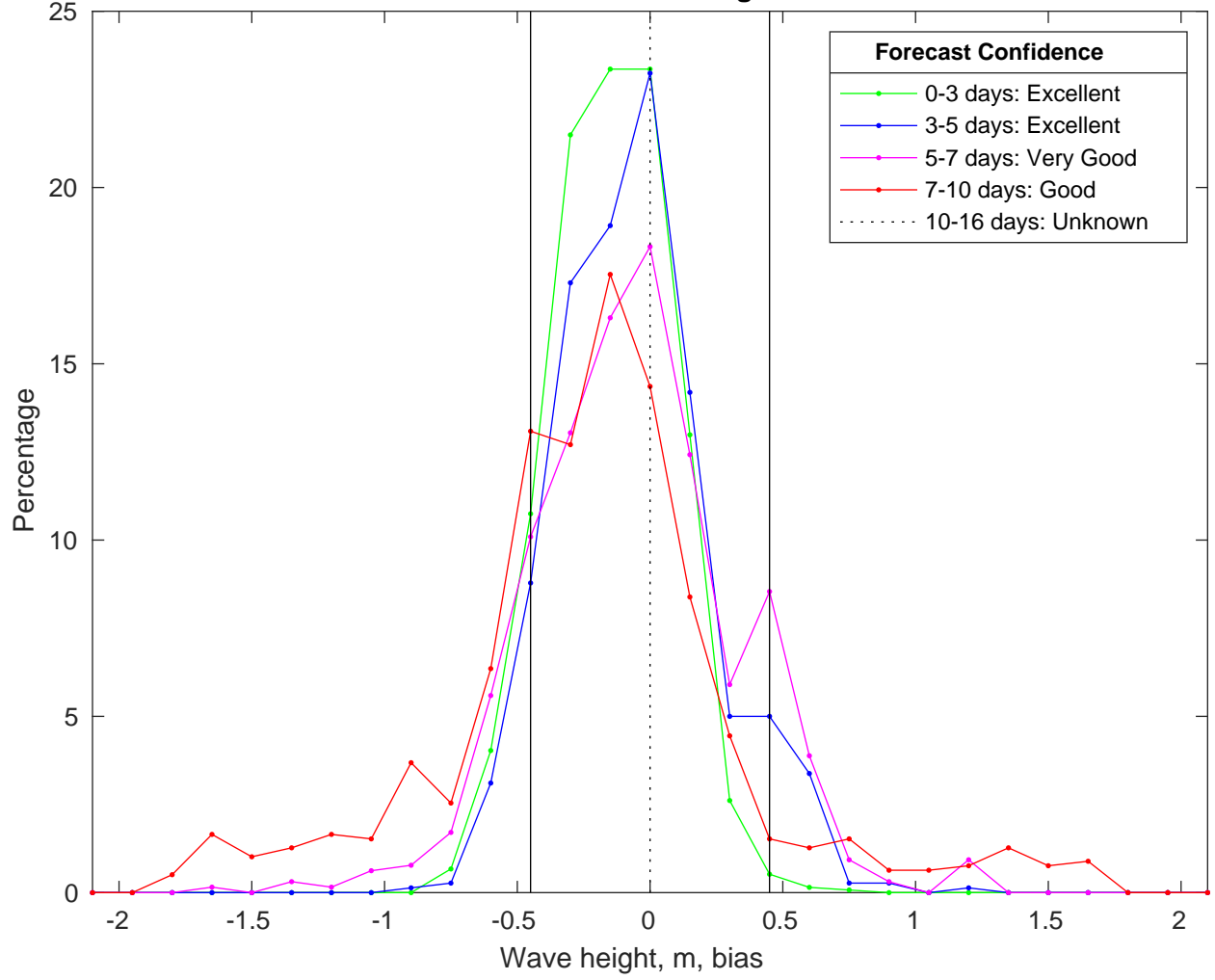
NDBC 46028 vs CMEMSWaves Bias Histogram: 21-Jan-2025
