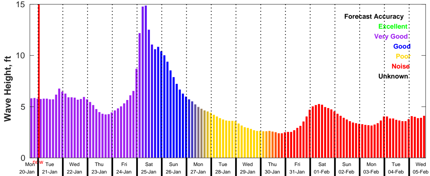
GFS Wave Forecast for NDBC 46028 from 20-Jan-2025 16:00:00 to 05-Feb-2025 16:00:00
