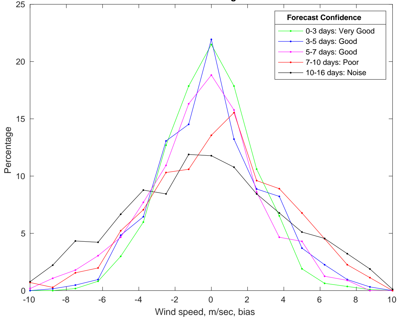
NDBC 46028 vs GFS Winds Bias Histogram: 26-Dec-2024
