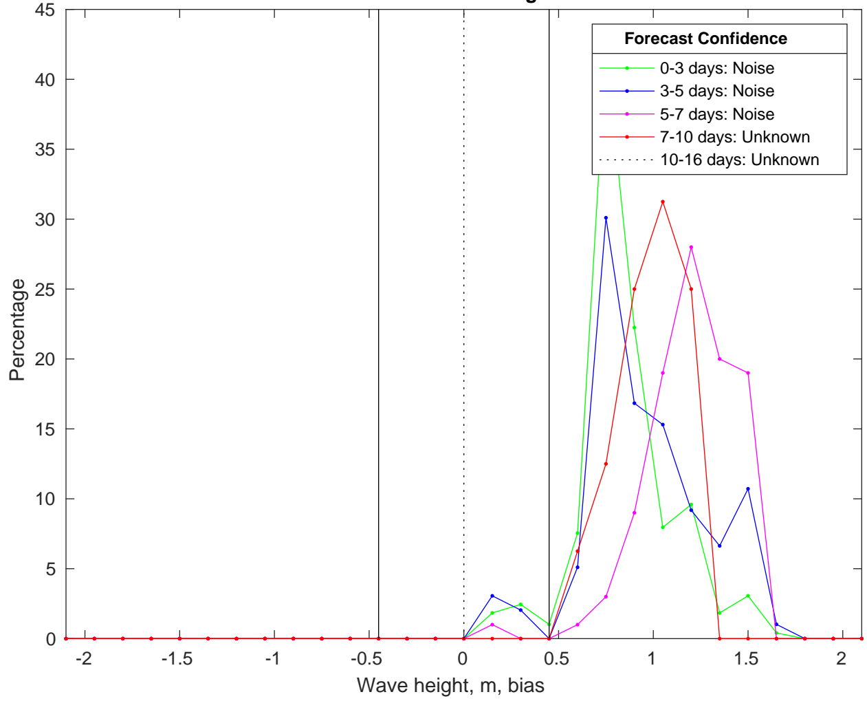
NDBC 46053 vs CMEMSWaves Bias Histogram: 21-Jan-2025
