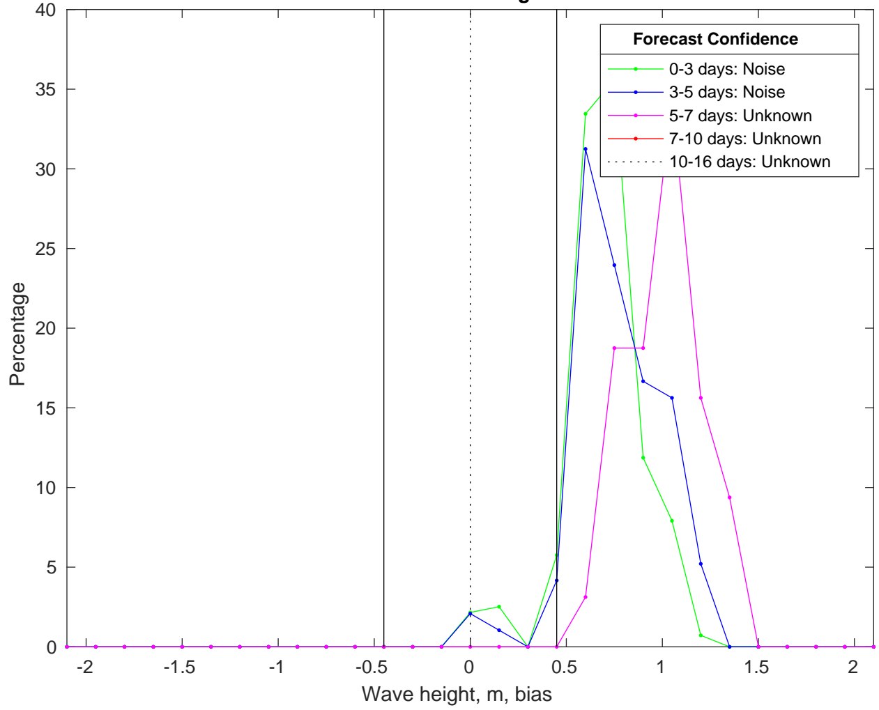
NDBC 46053 vs GFSWaves Bias Histogram: 21-Jan-2025
