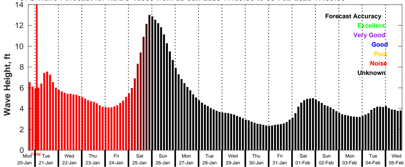
GFS Wave Forecast for NDBC 46053 from 20-Jan-2025 17:00:00 to 05-Feb-2025 17:00:00
