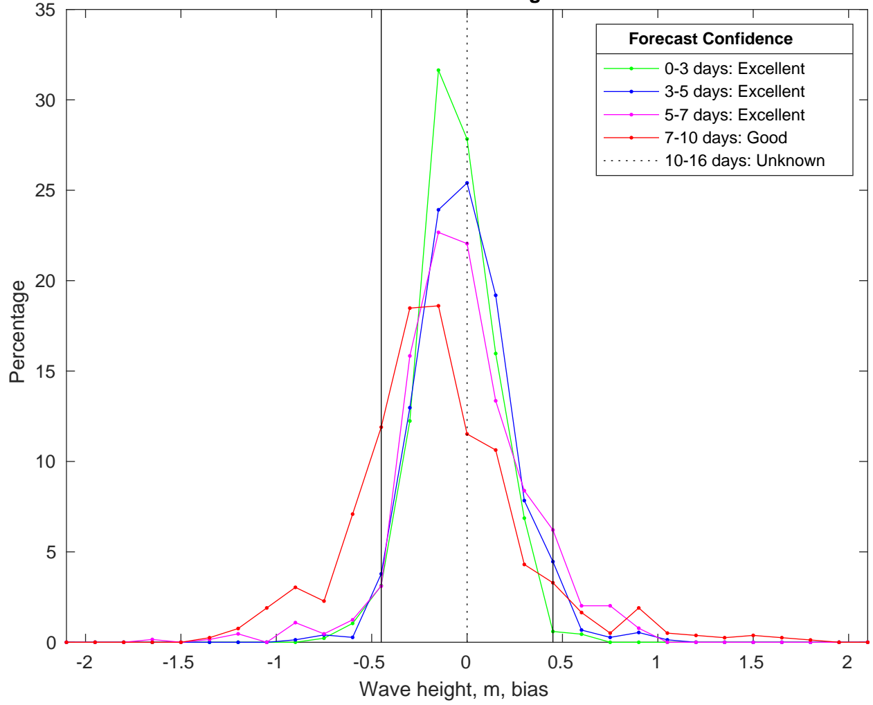
NDBC 46054 vs CMEMSWaves Bias Histogram: 21-Jan-2025
