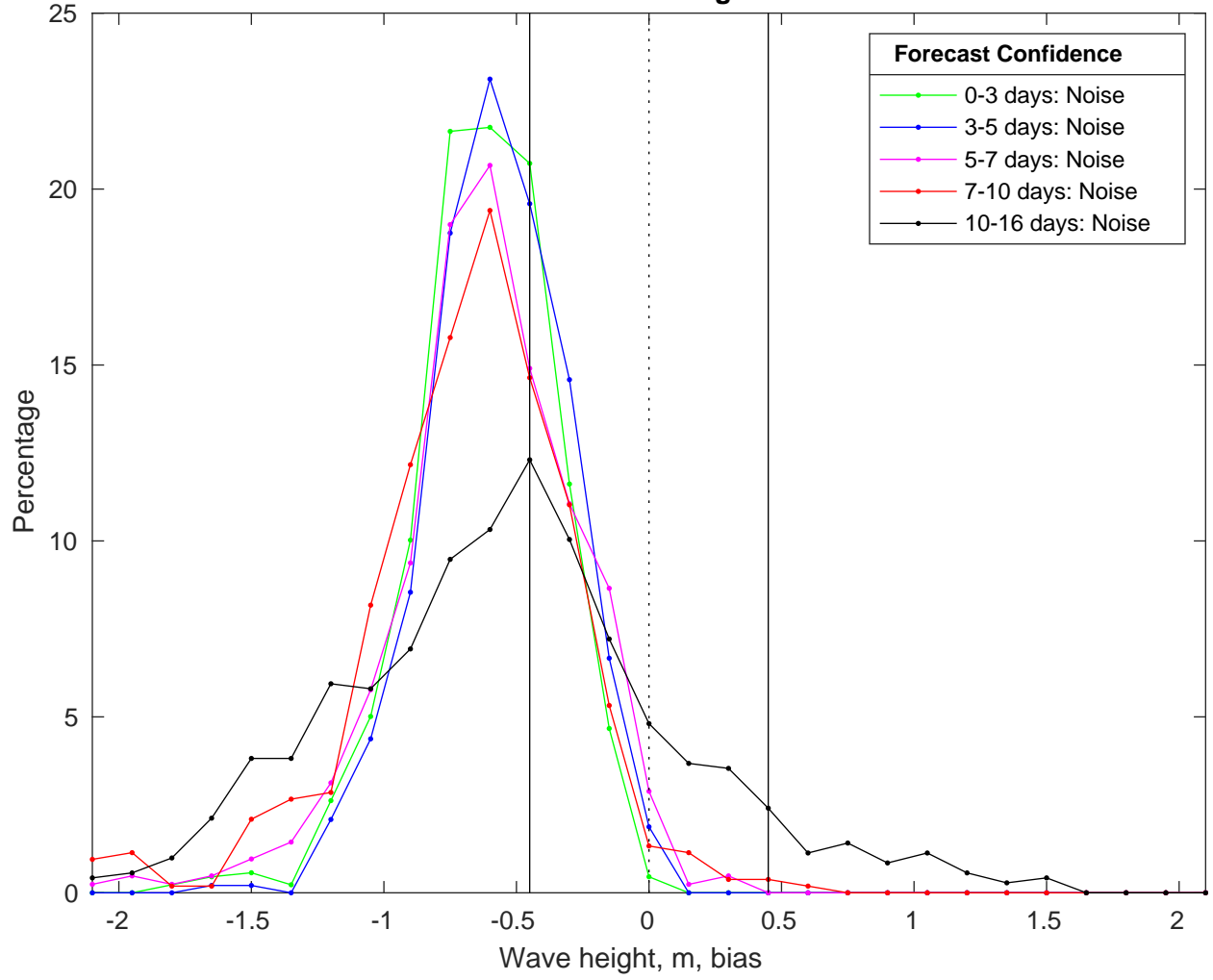
NDBC 46054 vs GFSWaves Bias Histogram: 21-Jan-2025
