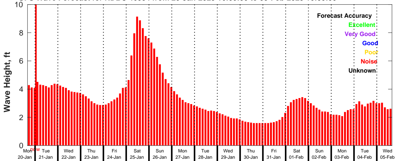
GFS Wave Forecast for NDBC 46054 from 20-Jan-2025 16:00:00 to 05-Feb-2025 16:00:00
