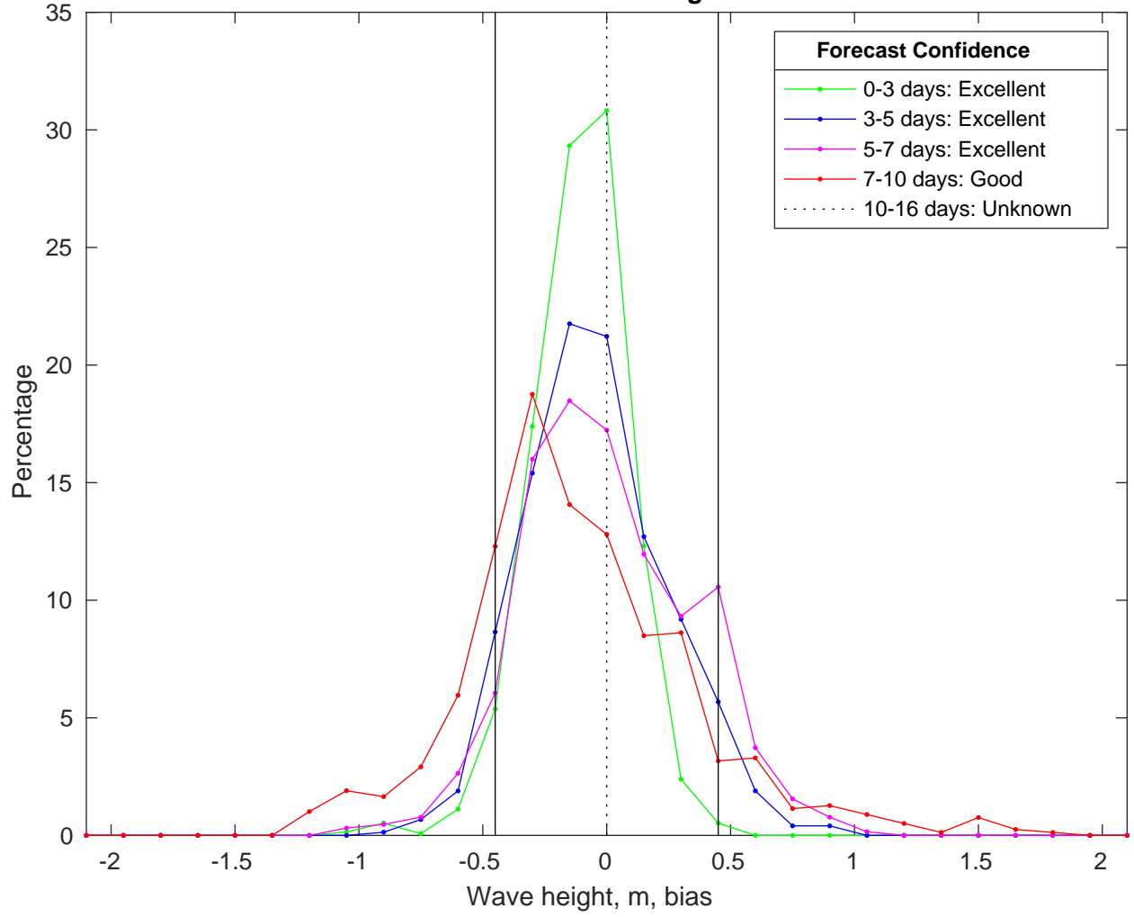
NDBC 46069 vs CMEMSWaves Bias Histogram: 21-Jan-2025
