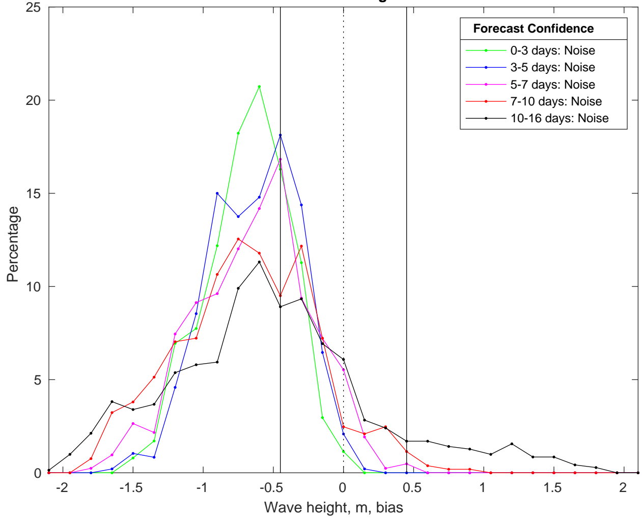
NDBC 46069 vs GFSWaves Bias Histogram: 21-Jan-2025
