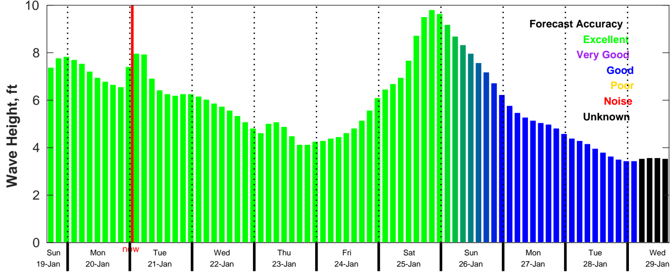
CMEMS Wave Forecast for NDBC 46069 from 19-Jan-2025 16:00:00 to 29-Jan-2025 16:00:00
