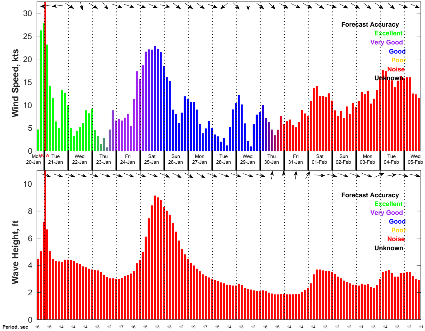
Wind & Wave Forecast for NDBC 46069 from 20-Jan-2025 16:00:00 to 05-Feb-2025 16:00:00
