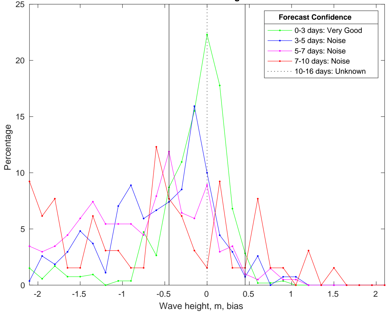
NDBC 46246 vs CMEMSWaves Bias Histogram: 21-Jan-2025
