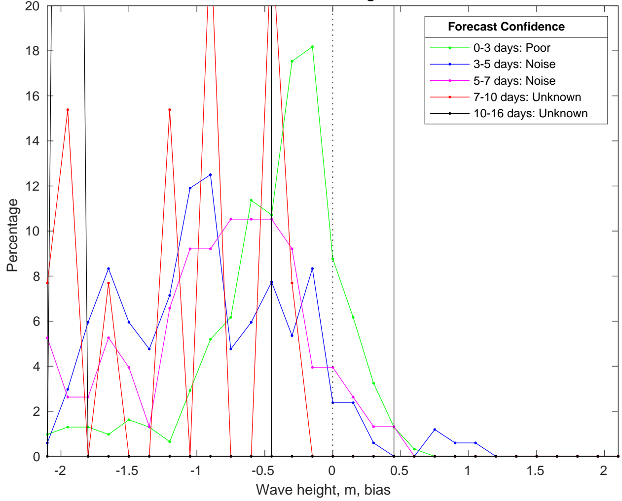
NDBC 46246 vs GFSWaves Bias Histogram: 21-Jan-2025
