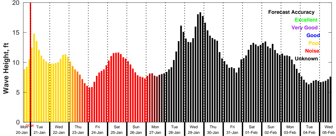
GFS Wave Forecast for NDBC 46246 from 20-Jan-2025 15:00:00 to 05-Feb-2025 15:00:00
