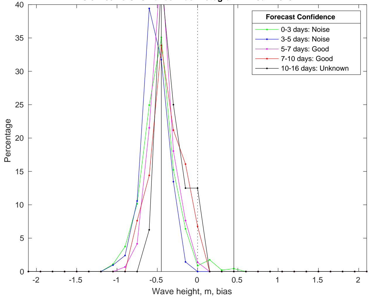
NDBC 51209 vs GFSWaves Bias Histogram: 21-Jan-2025
