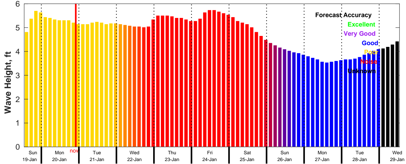
CMEMS Wave Forecast for NDBC 51209 from 19-Jan-2025 13:00:00 to 29-Jan-2025 13:00:00
