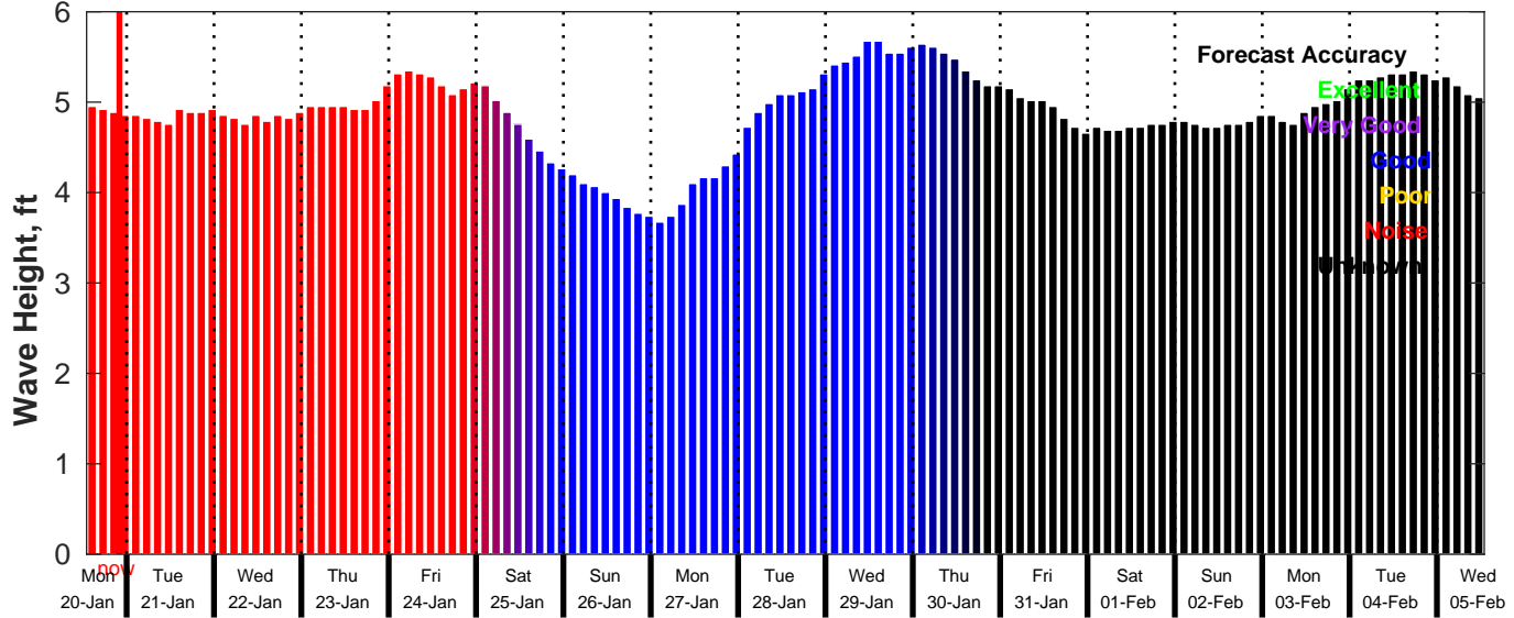
GFS Wave Forecast for NDBC 51209 from 20-Jan-2025 13:00:00 to 05-Feb-2025 13:00:00
