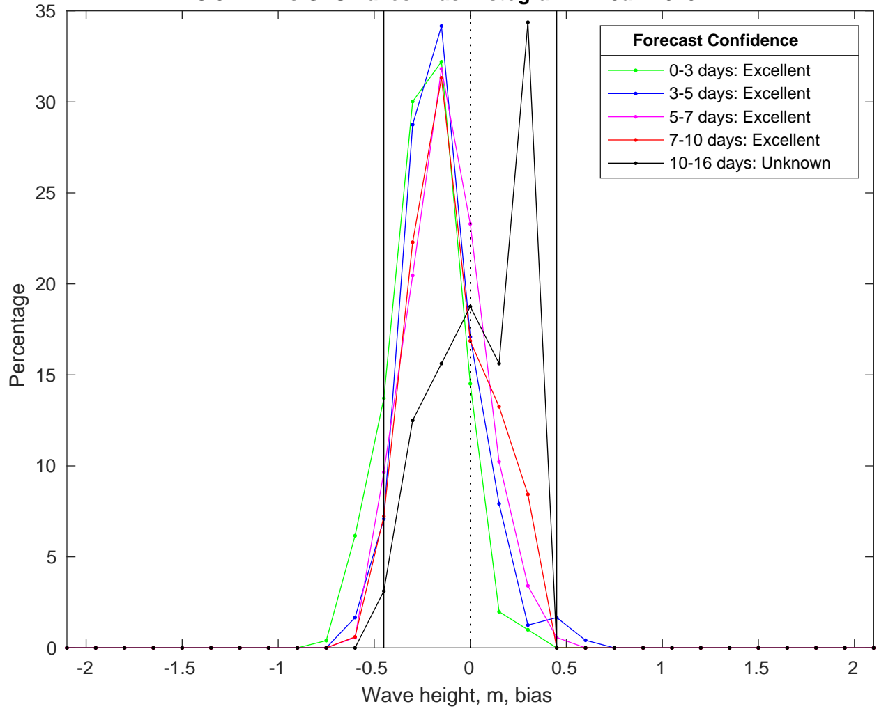
NDBC 52212 vs GFSWaves Bias Histogram: 21-Jan-2025
