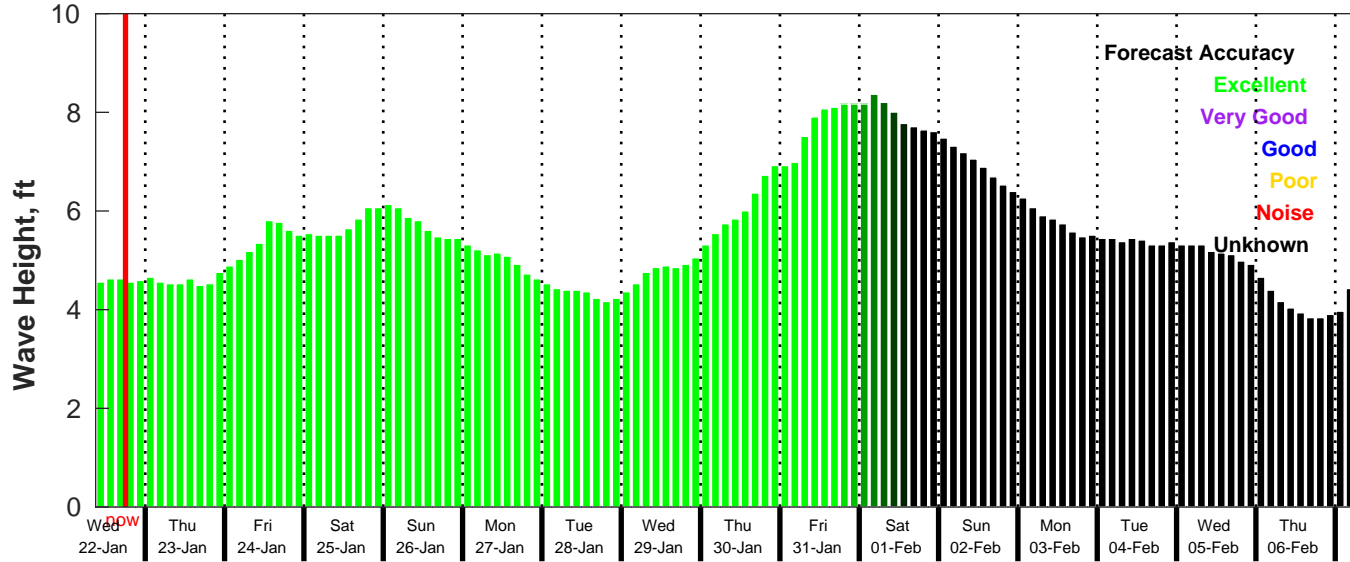
GFS Wave Forecast for NDBC 52212 from 21-Jan-2025 09:00:00 to 06-Feb-2025 09:00:00
