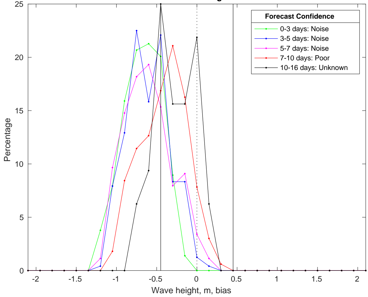
NDBC 52213 vs GFSWaves Bias Histogram: 21-Jan-2025
