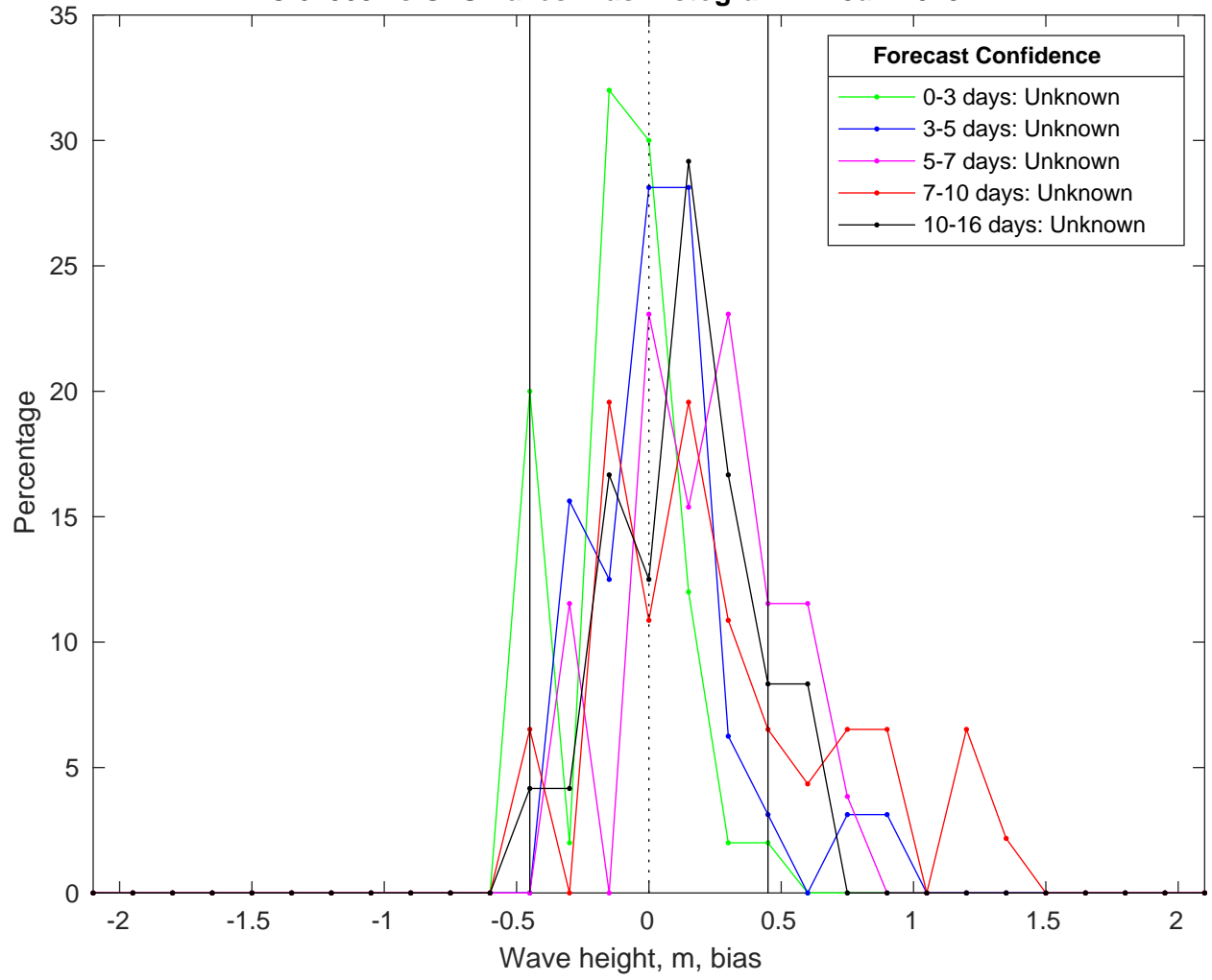
NDBC 62305 vs GFSWaves Bias Histogram: 21-Jan-2025
