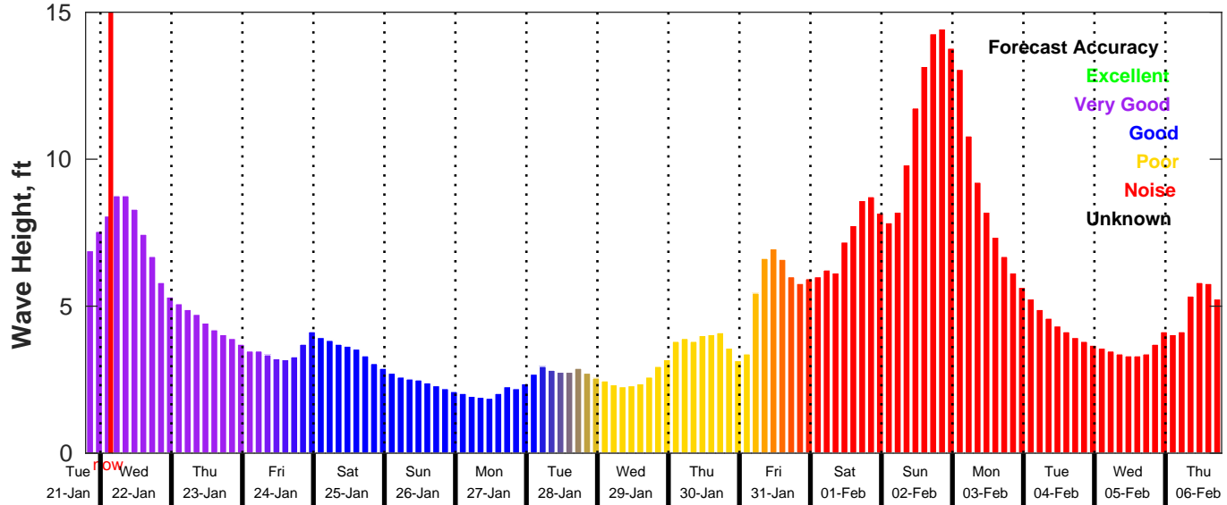
GFS Wave Forecast for NDBC 41004 from 21-Jan-2025 19:00:00 to 06-Feb-2025 19:00:00
