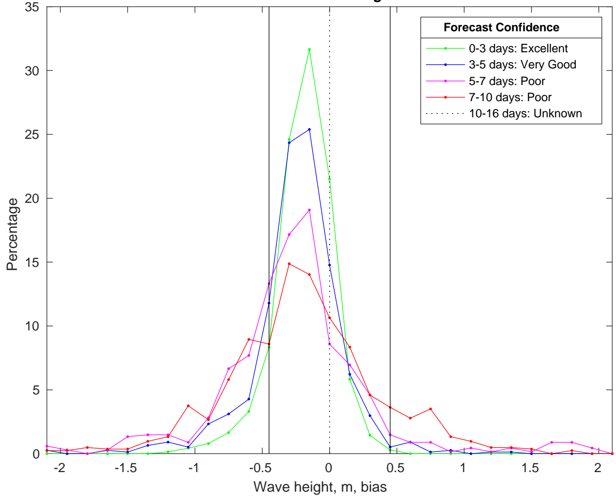
NDBC 41013 vs CMEMSWaves Bias Histogram: 22-Jan-2025
