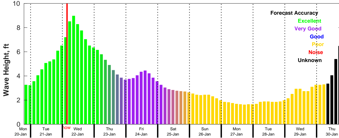
CMEMS Wave Forecast for NDBC 41013 from 20-Jan-2025 19:00:00 to 30-Jan-2025 19:00:00
