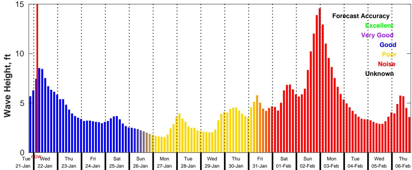
GFS Wave Forecast for NDBC 41013 from 21-Jan-2025 19:00:00 to 06-Feb-2025 19:00:00
