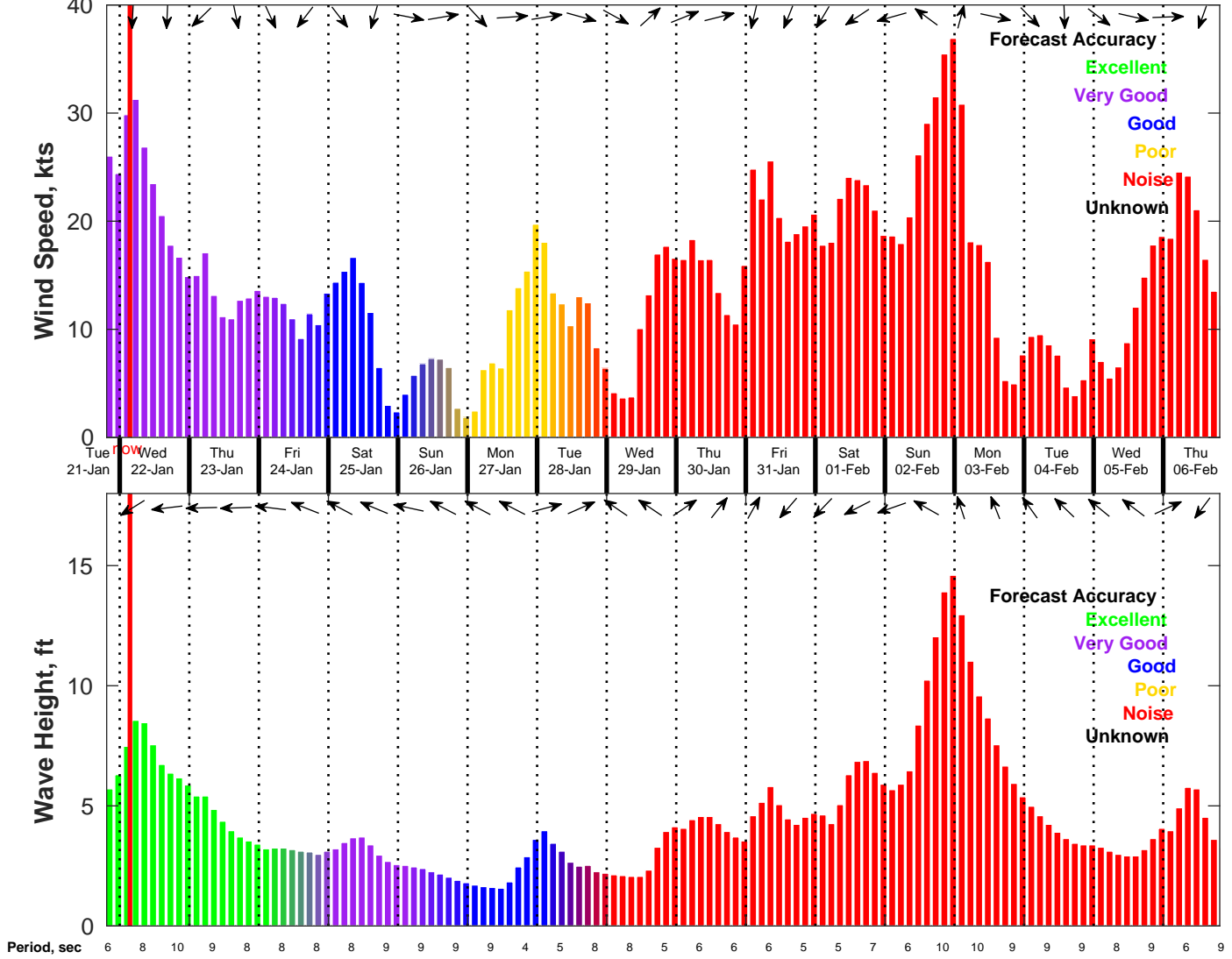
Wind & Wave Forecast for NDBC 41013 from 21-Jan-2025 19:00:00 to 06-Feb-2025 19:00:00
