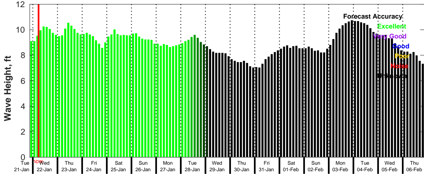
GFS Wave Forecast for NDBC 41040 from 21-Jan-2025 21:00:00 to 06-Feb-2025 21:00:00
