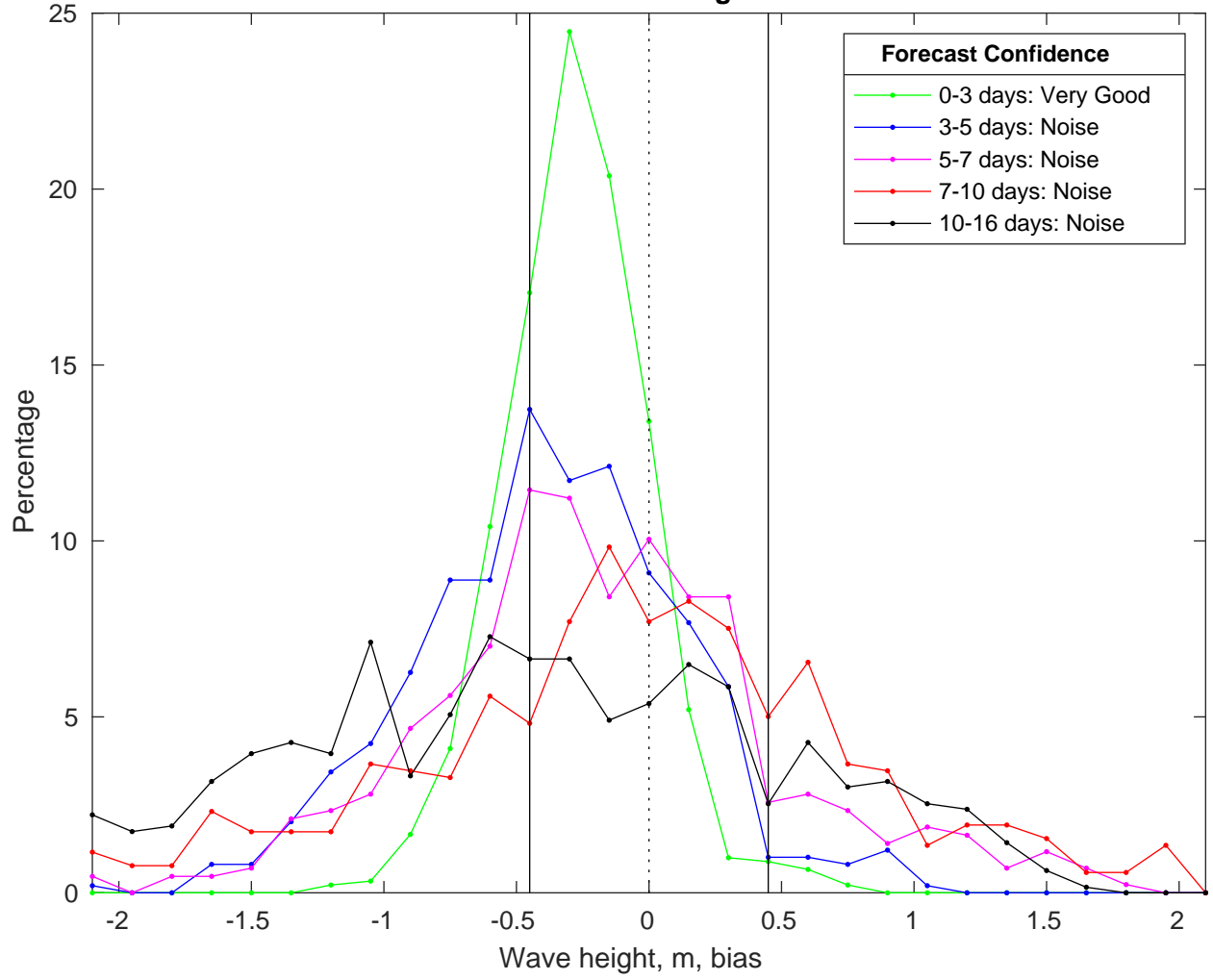
NDBC 42019 vs GFSWaves Bias Histogram: 22-Jan-2025
