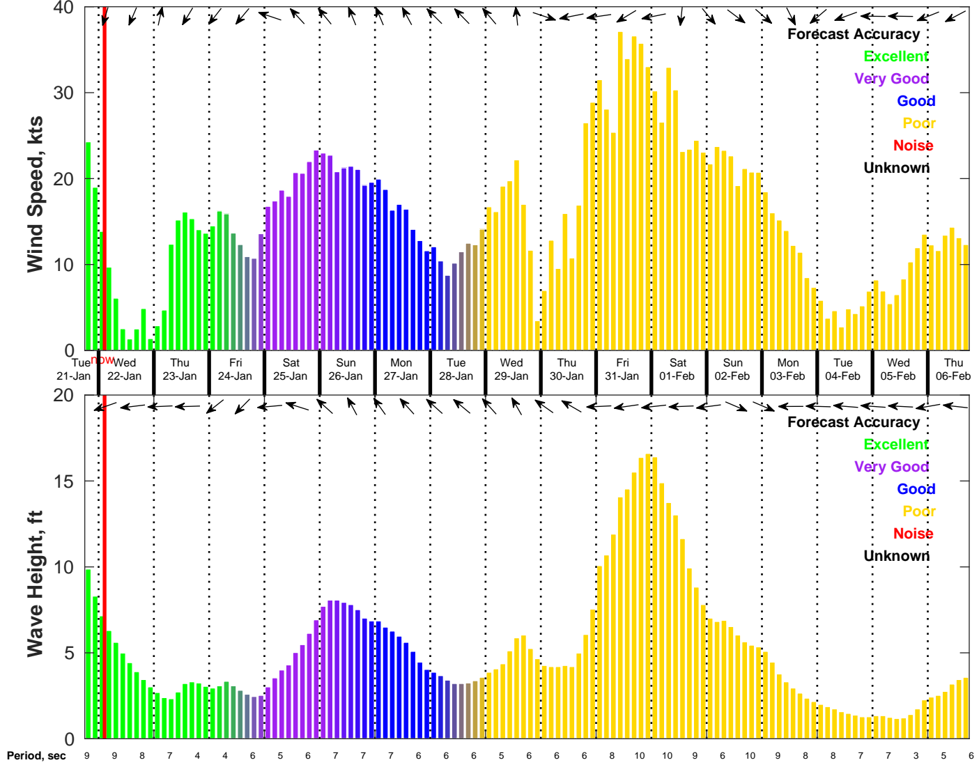
Wind & Wave Forecast for NDBC 42019 from 21-Jan-2025 18:00:00 to 06-Feb-2025 18:00:00
