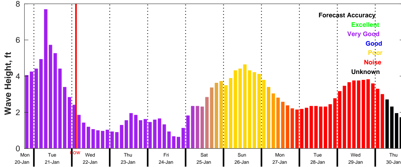
CMEMS Wave Forecast for NDBC 42035 from 20-Jan-2025 18:00:00 to 30-Jan-2025 18:00:00
