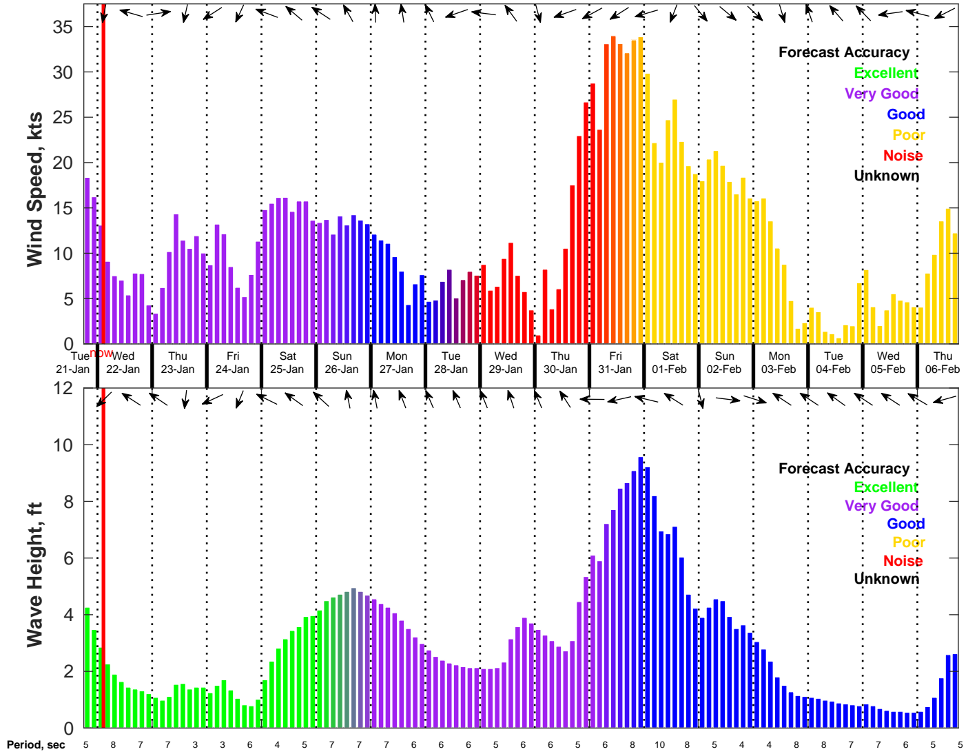
Wind & Wave Forecast for NDBC 42035 from 21-Jan-2025 18:00:00 to 06-Feb-2025 18:00:00
