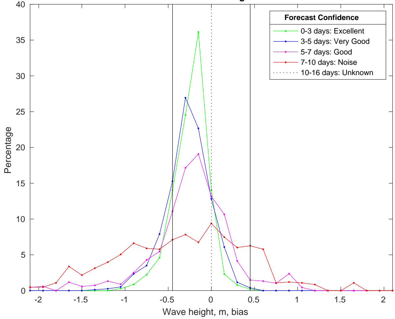
NDBC 42036 vs CMEMSWaves Bias Histogram: 22-Jan-2025
