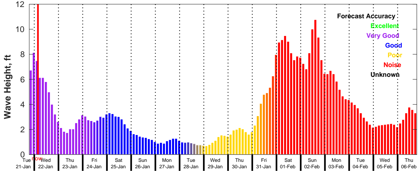
GFS Wave Forecast for NDBC 42036 from 21-Jan-2025 19:00:00 to 06-Feb-2025 19:00:00
