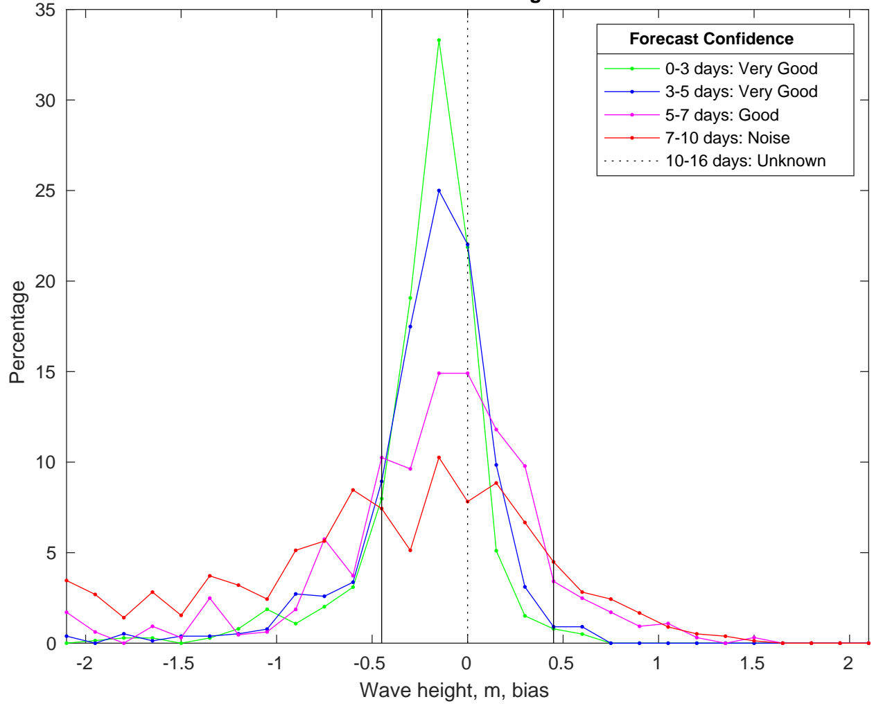
NDBC 42040 vs CMEMSWaves Bias Histogram: 22-Jan-2025
